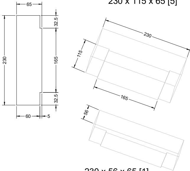
230 x 56 x 65 [1]
