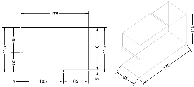
175 x 115 x 65 [2]
